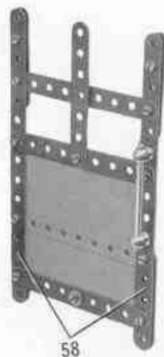
FIG. 10 Detail of the sliding door of the cab
