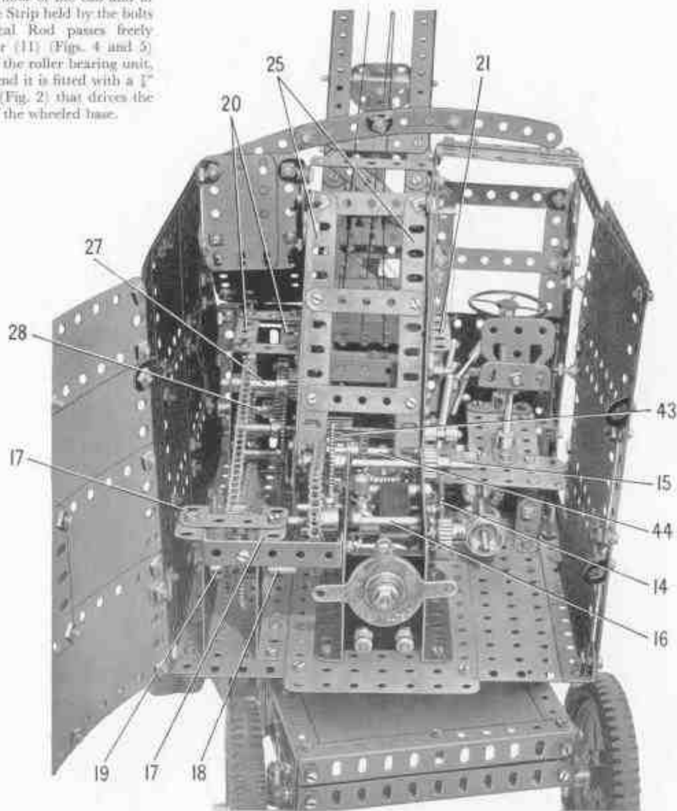
FIG. 7 A view of the general layout inside the cab
