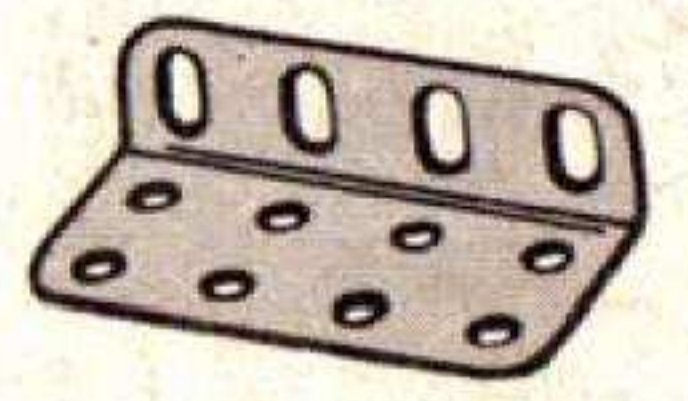
GIRDER BRACKET 161 - 2" x 1" x 1/2"; 50 x 25 x 12 mm
