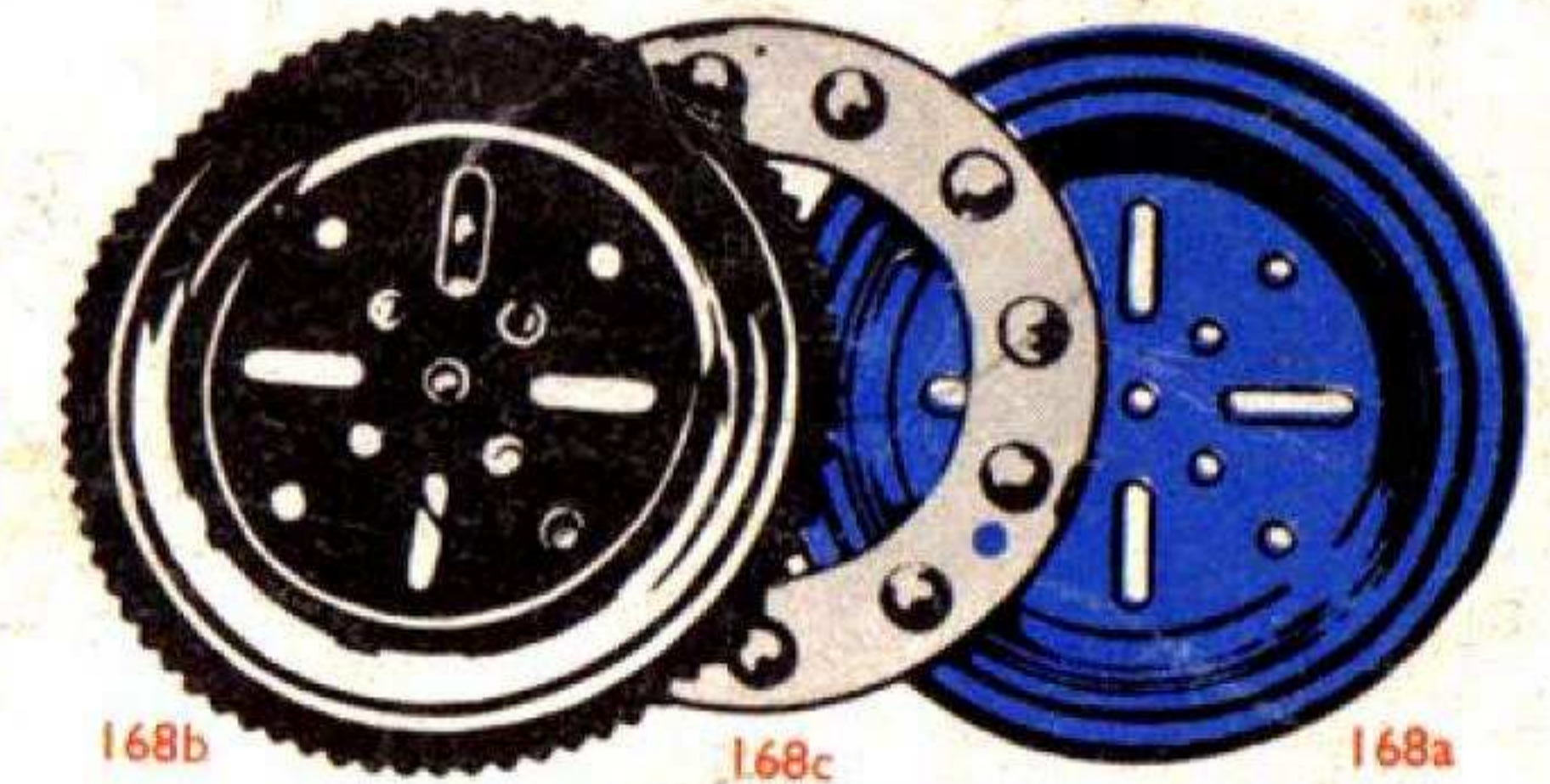
168 BALL THRUST BEARING COMPLETE 4"; 10 cm 168a AND 168b BALL THRUST RACES 168c BALL CAGE
