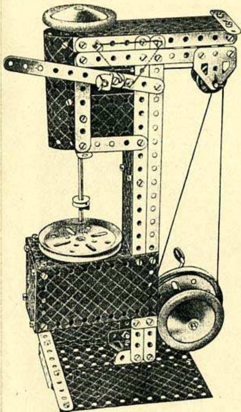
Perforeuse
