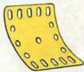
CURVED PLATE 200 - 2 1/2" x 2 1/2" x 1 1/8"; 60 x 60 x 43 mm
