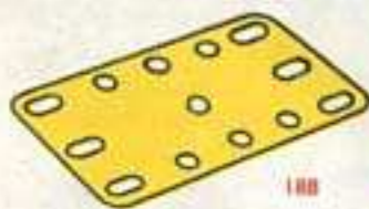
FLEXIBLE PLATES 188 - 2 1/2" x 1 1/2"; 60 x 38 mm 189 - 5" x 1 1/2"; 140 x 38 mm 190 - 2 1/2" x 2 1/2"; 6 x 6 cm 190a - 3 1/2" x 2 1/2"; 9 x 6 cm 191 - 4 1/2" x 2 1/2"; 11 1/2 x 6 cm 192 - 5 1/2" x 2 1/2"; 14 x 6 cm
