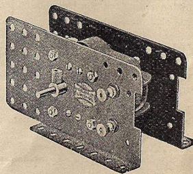
Meccano Electromotor No. E20A
