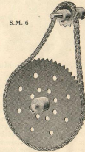
S.M. 6—Chain Gear \frac{3}{4} " and 3" diam. Sprocket Wheels. Ratio, 4 : 1. 1" and 2" diam. Sprocket Wheels. Ratio, 2 : 1. \frac{3}{4} " and 1\frac{1}{2} " diam. Sprocket Wheels. Ratio, 2 : 1. etc., etc. Ratios of 1 : 1 may be obtained by gearing any two Sprocket Wheels of like diameter.
