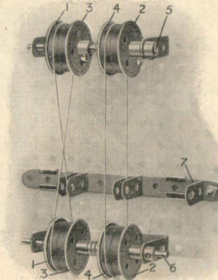
S.M. 18—Belt Reversing Gear. Two pairs of Flanged Wheels, 1 and 2, are fixed, and two pairs, 3 and 4, are loose on a driving shaft 5 and a driven shaft 6. The wheels 1 are connected by a crossed belt, thereby reversing the motion of the driven shaft 6 (as in S.M.17), while the wheels 4 are connected by an open belt. The operation of a lever 7 brings one of the belts on to a pair of fixed pulleys, at the same time throwing the other on to a loose pair, or vice versa, thereby reversing the action of the driven shaft 6.
