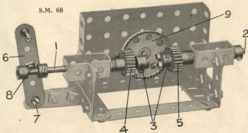
S.M. 68—REVERSING GEAR
