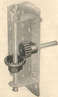
S.M. 4—Contrate Gear \frac{1}{2} " Pinion and \frac{3}{4} " Contrate Wheel. Ratio, Approx. 1\frac{1}{2} : 1.
