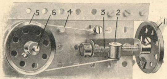
S.M. 105—STRAP AND SCREW BRAKE
