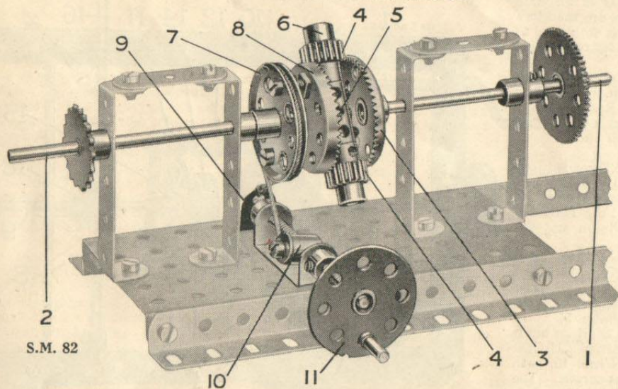
S.M. 82—EPICYCLIC GEAR CLUTCH
