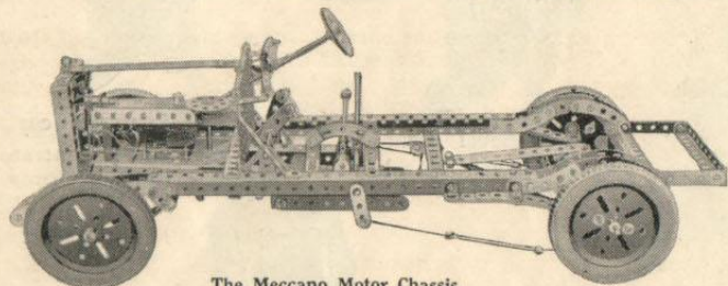
The Meccano Motor Chassis complete with Gear Box, Clutch, Differential and Ackermann Steering
