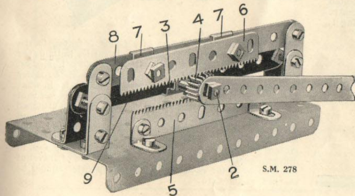
S.M. 278—DEVICE TO INCREASE LENGTH OF A CRANK STROKE
