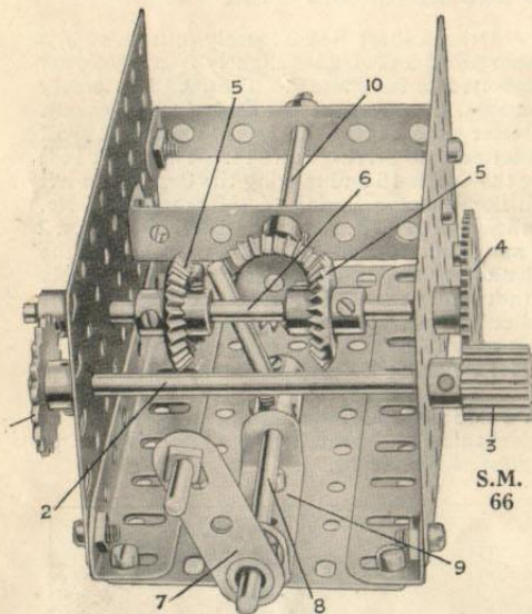
S.M. 66—BEVEL REVERSING GEAR
