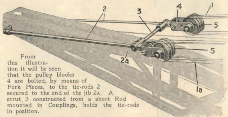
S.M. 43—PULLEY BLOCKS PIVOTED TO JIB-HEAD
