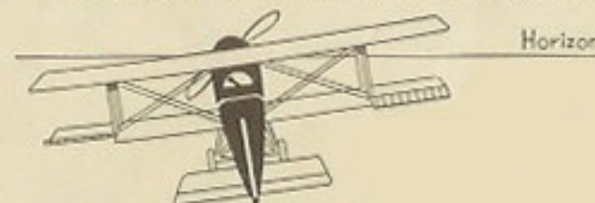
When the stick is moved over to the left, the ailerons on that side are raised and the wings drop, producing left bank.
