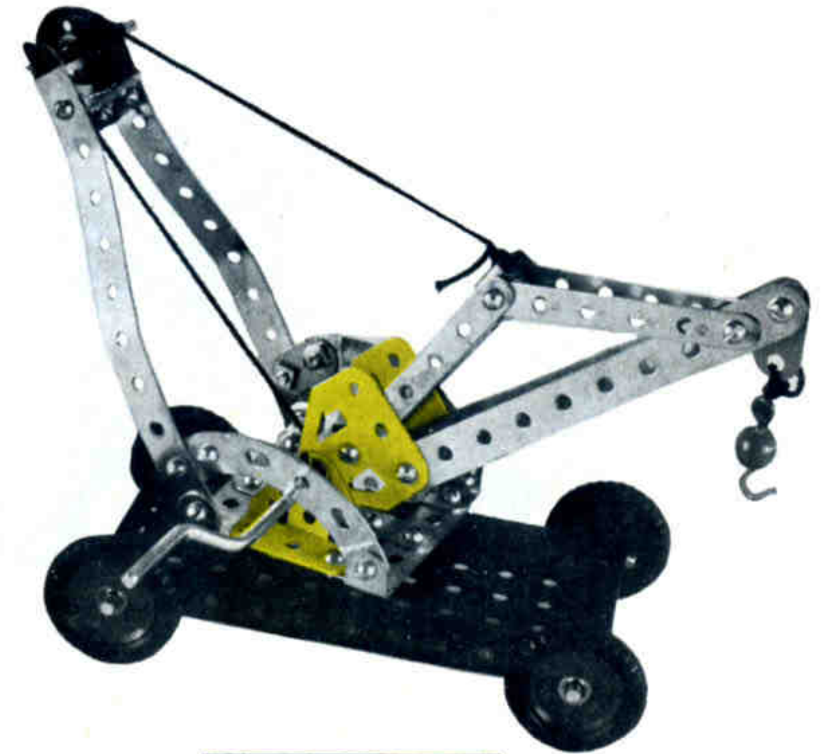
111 Moveable crane Grue mobile Gru mobile Beweglicher Kran Guindaste móvel
